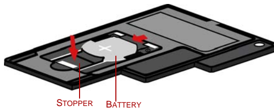
Figure 2-20 Removing the batteries
